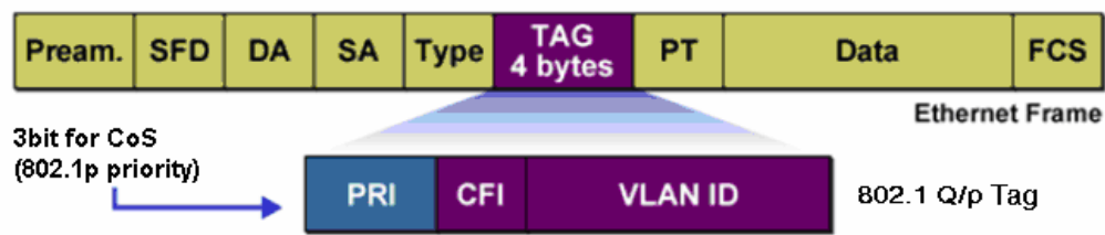
Figure 9-2 802.1Q frame
